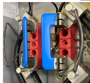
Uncoated Blades JMP-UB
