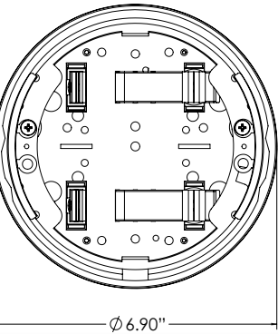
Meter Socket Form Converter CNV-LP-16S-01/02S
