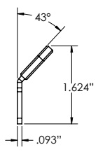
Coated, Angled JMP-CA-04
