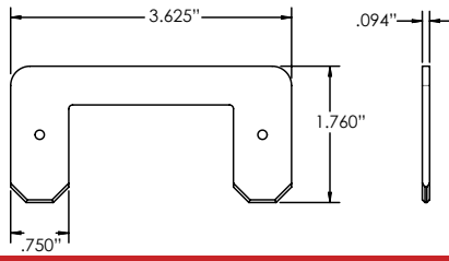
Uncoated Blades JMP-UB
